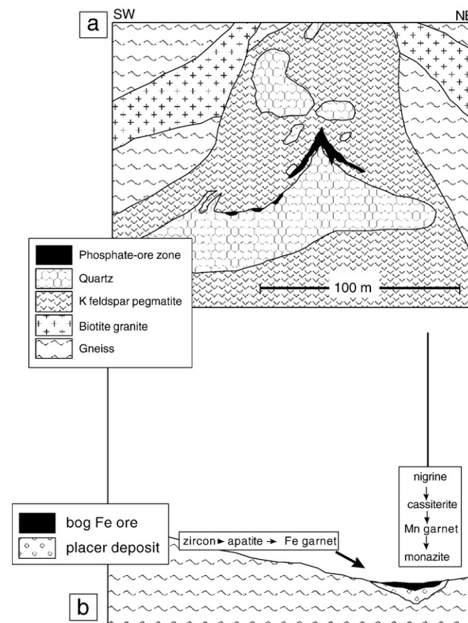
Fig. 3. Mineral deposits in the Pleystein area. a) The late Variscan Li–Fe–Mn phosphate-bearing pegmatite Hagendorf South, reference type of pegmatites in the Hagendorf–Pleystein Pegmatite Province (redrawn from Strunz et al. 1976). b) Tin and titanium alluvial–fluvial Quaternary placer deposits with accessory minerals and their provenance areas (Dill et al. 2008). The arrows denote where the minerals in the boxes came from (vertical: pegmatite, horizontal: metamorphic country rocks). On top of these placer deposits and blanketing the overbank deposits of the channels, bog iron ores formed during the Quaternary.
