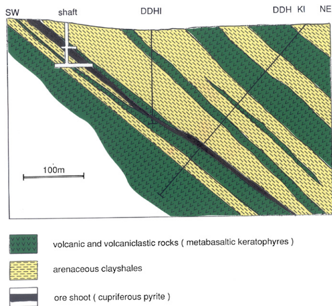
Fig. 4. Mineral deposits in the Kupferberg area. Stratabound-stratiform pyrite-chalcocopyrite deposits of Besshi-Type/VMS-Type (volcanic massive sulfide). For location see Fig. 1.
